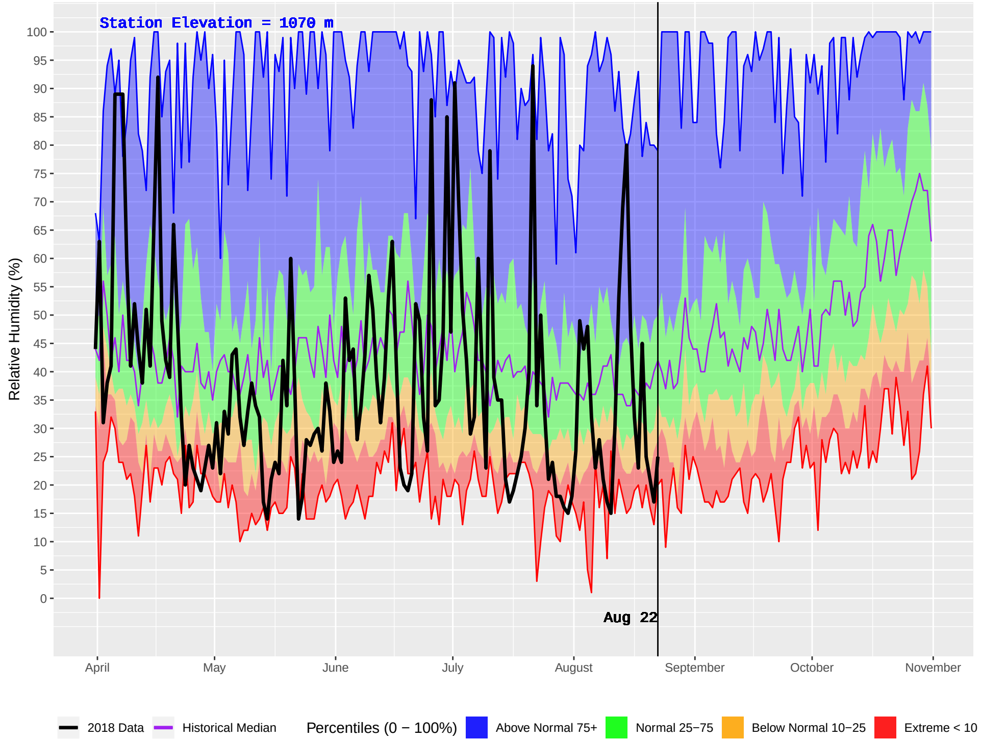
MEADOW LAKE (236) : Historical (1991–2016) and Current (2018) Daily Relative Humidity
