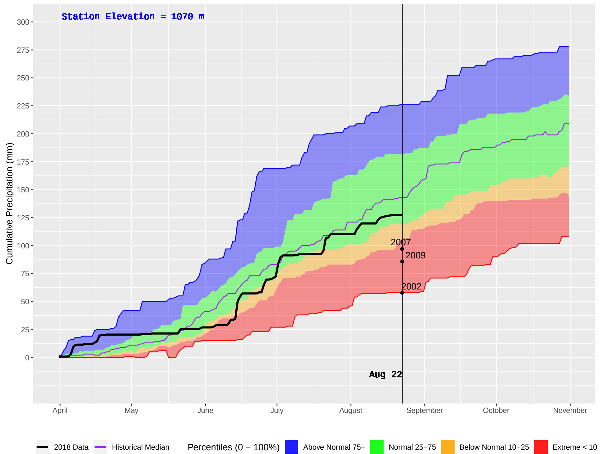
MEADOW LAKE (236) : Historical (1991–2016) and Current (2018) Daily Cumulative Precipitation
