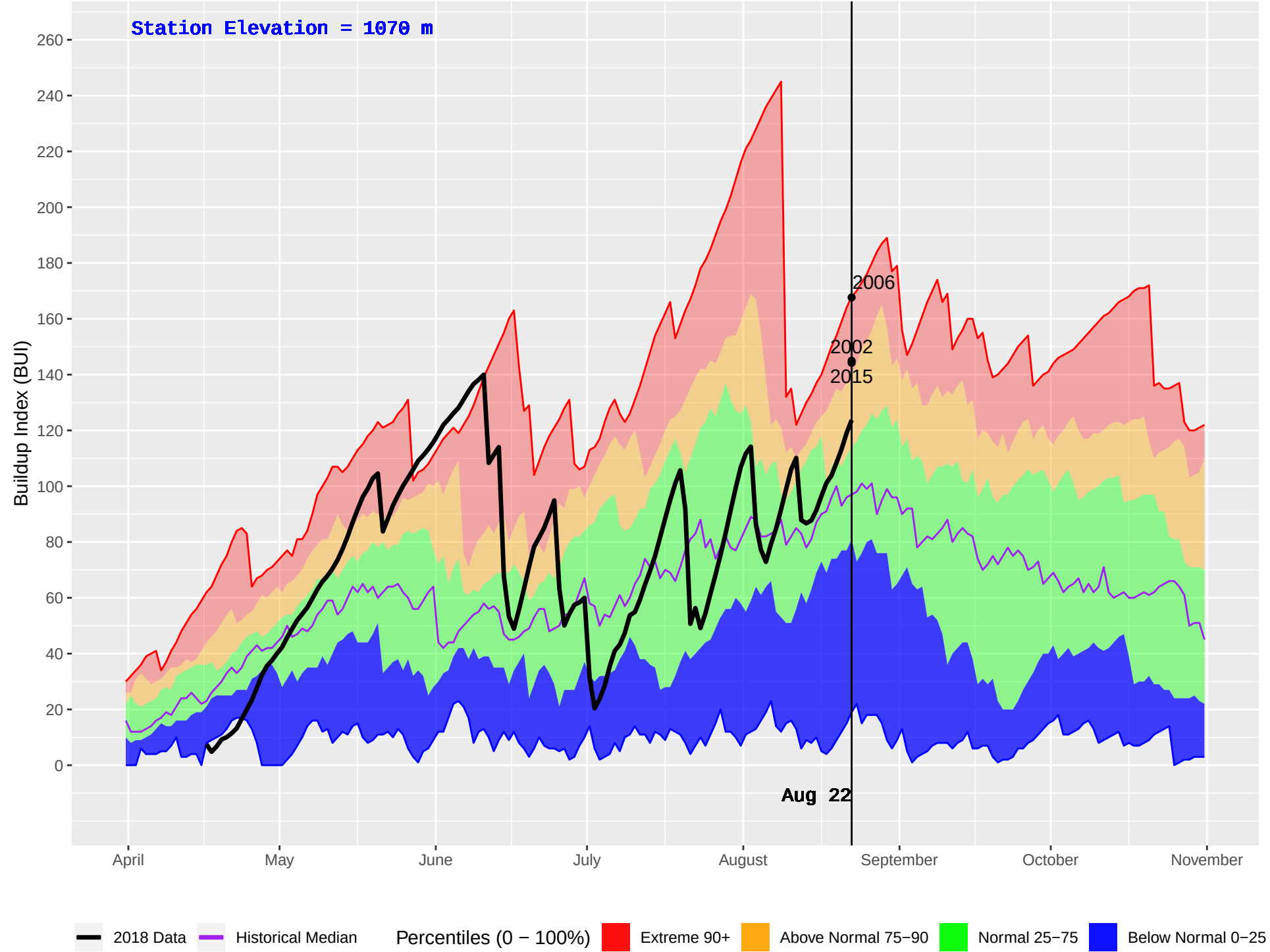
MEADOW LAKE (236) : Historical (1991–2016) and Current (2018) Daily Buildup Index (BUI)
