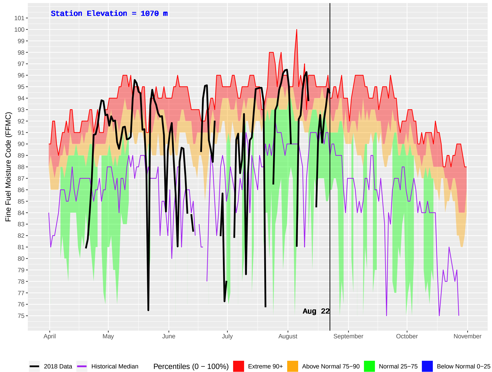
MEADOW LAKE (236) : Historical (1991–2016) and Current (2018) Daily Fine Fuel Moisture Code (FFMC)
