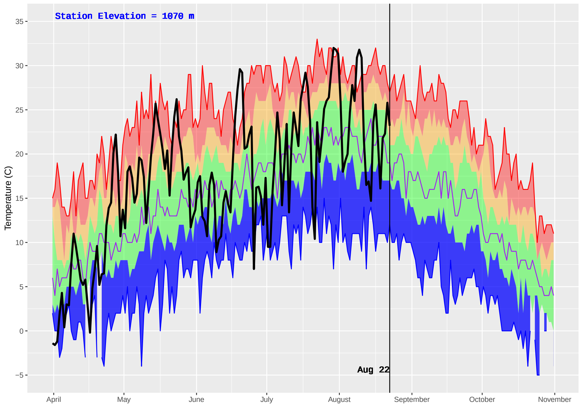
MEADOW LAKE (236) : Historical (1991–2016) and Current (2018) Daily Temperature
