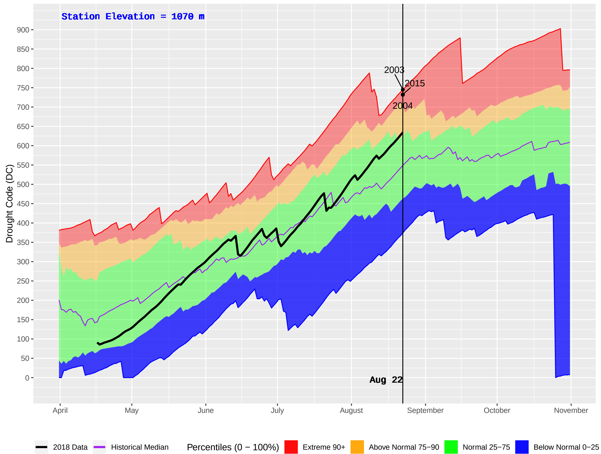
MEADOW LAKE (236) : Historical (1991–2016) and Current (2018) Daily Drought Code (DC)
