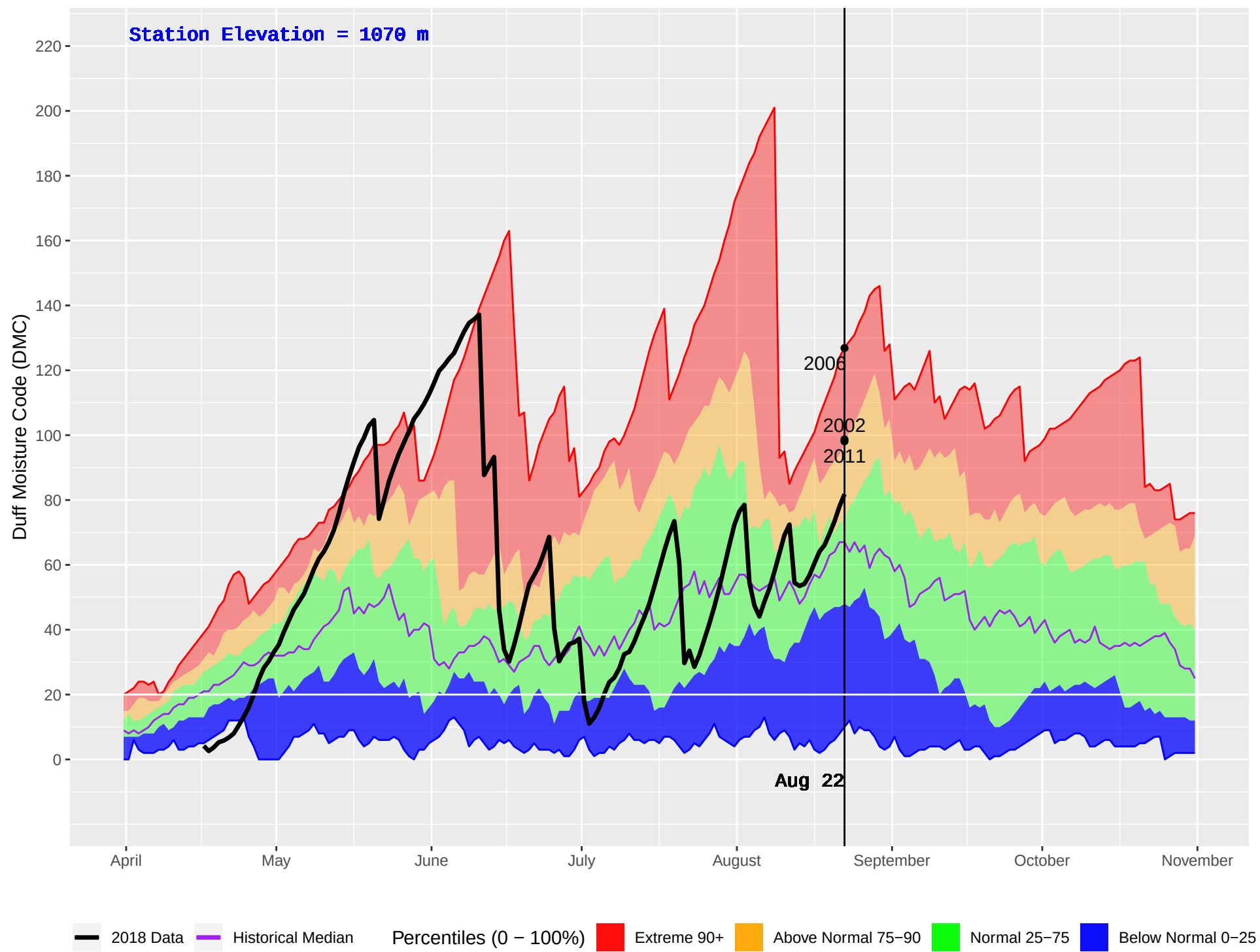
MEADOW LAKE (236) : Historical (1991–2016) and Current (2018) Daily Duff Moisture Code (DMC)
